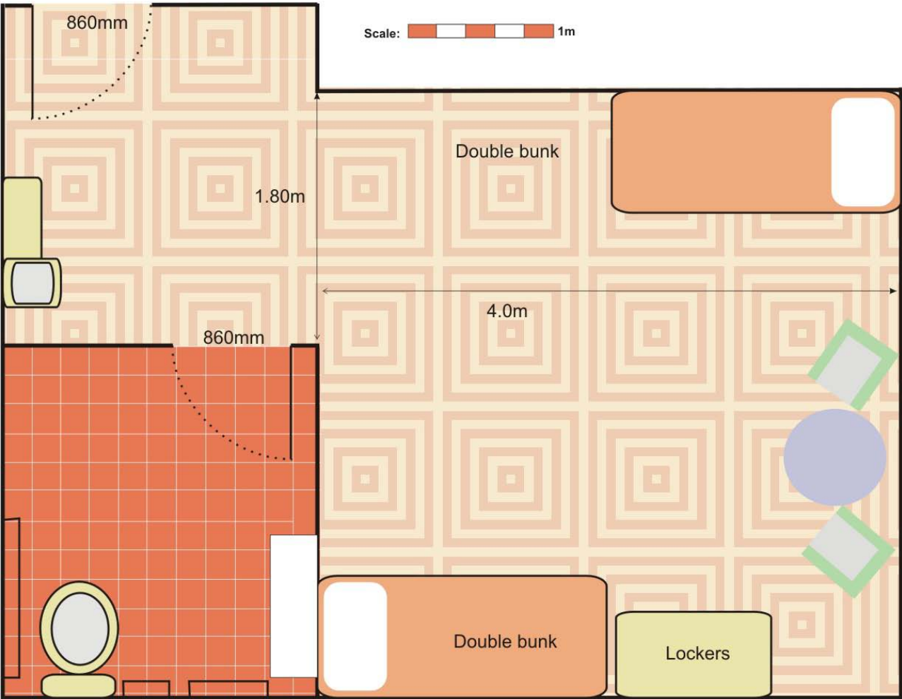
Floorplan Accessible Room 119
